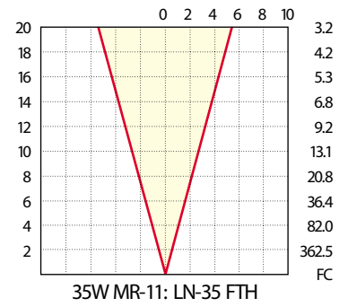
Beam Spread: 30
