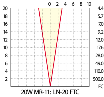
Beam Spread: 17
