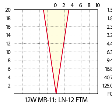
Beam Spread: 17
