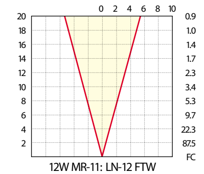
Beam Spread: 30
