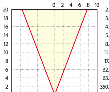
35W MR-16: LN-35 FMW
