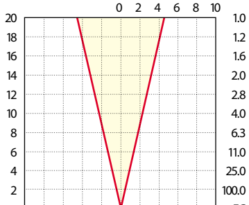
10W MR-16: LN-10 ALR
