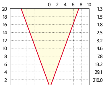
20W MR-16: LN-20 BAB
