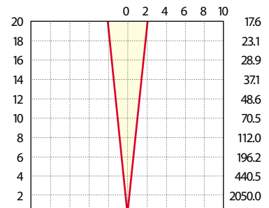
35W MR-16: LN-35 FMT
