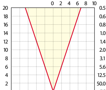
10W MR-16: LN-10 AEC
