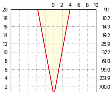
35W MR-16: LN-35 FMV
