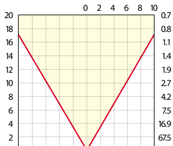
20W MR-16: LN-20 BAB/60
