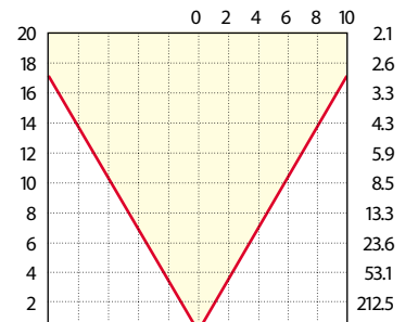
35W MR-16: LN-35 FMW/60
