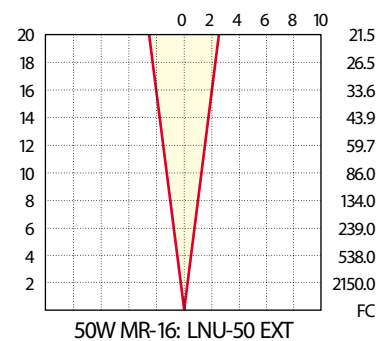
Beam Spread: 12
