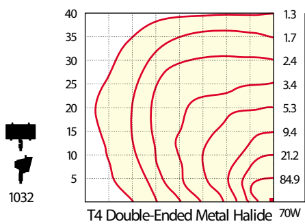
Horizontal Foot Candle Half Spread
