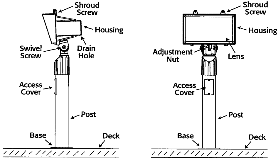
Fixture shown in optional Stanchion Mount configuration with CM150 Top Mount and SM118 Mounting Post
